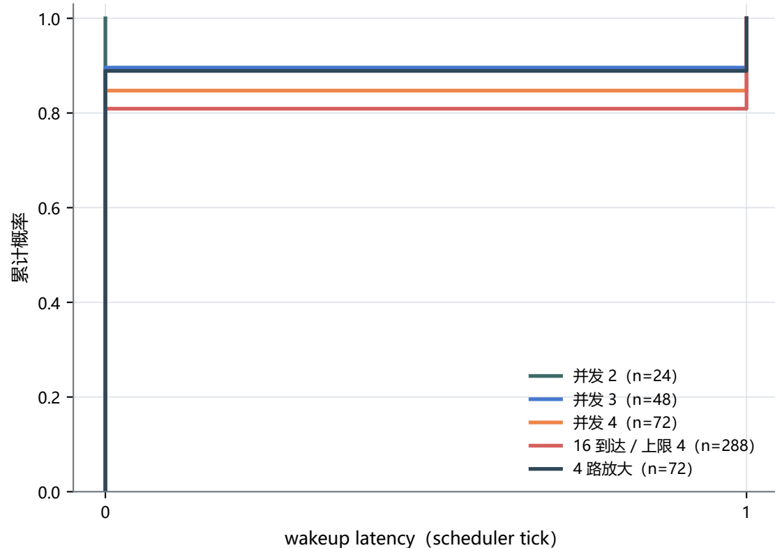
EEVDF 精确 wakeup latency ECDF
