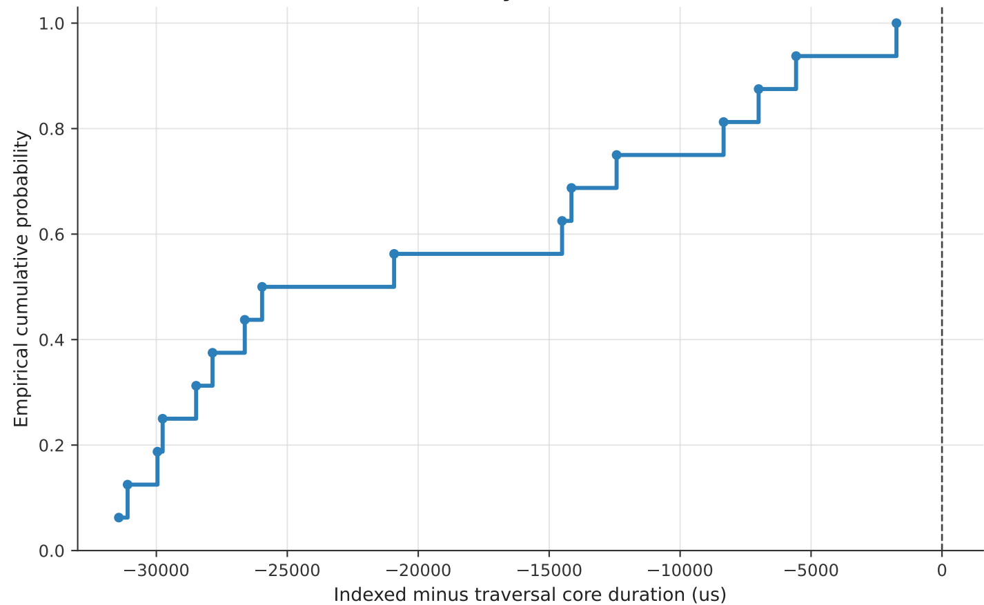
Paired latency difference ECDF
