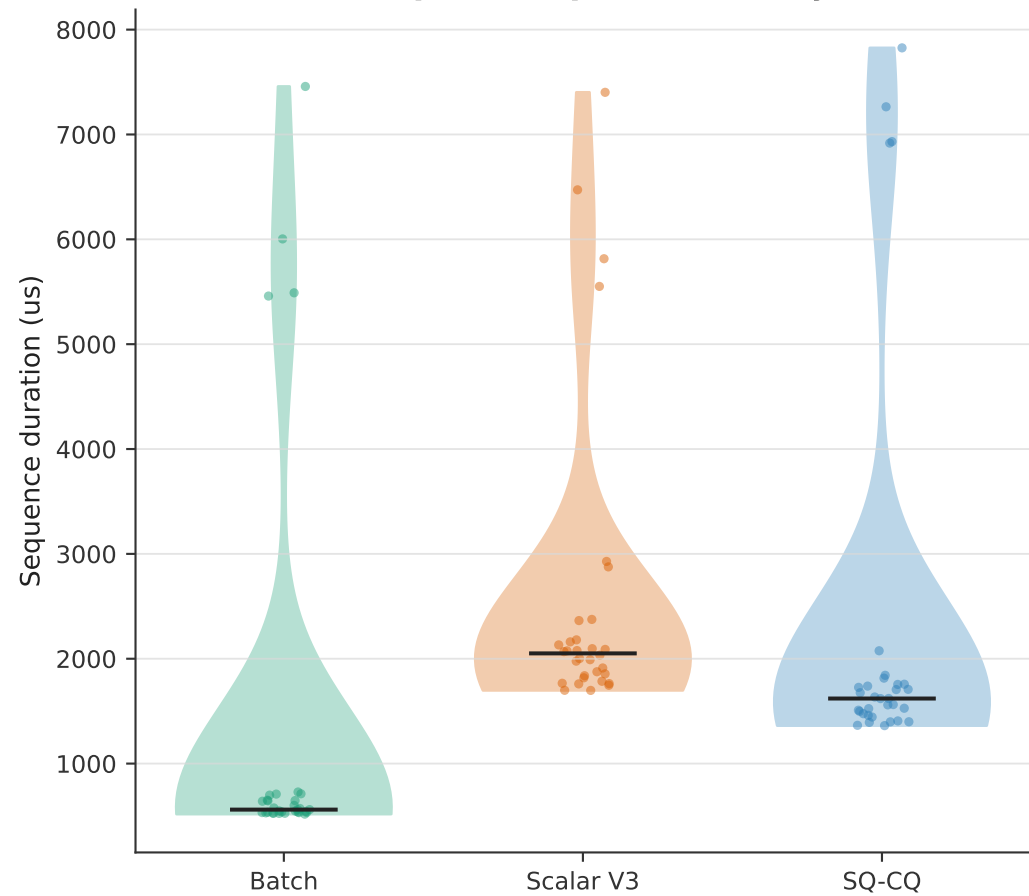
Complete sequence latency
