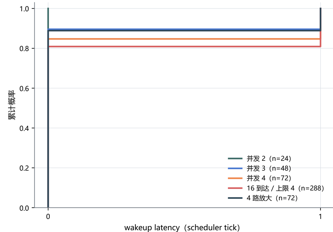
EEVDF wakeup latency ECDF
