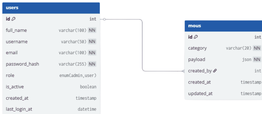
Gambar 2.4 Entity Relationship Diagram (ERD) Database SIKERMA
