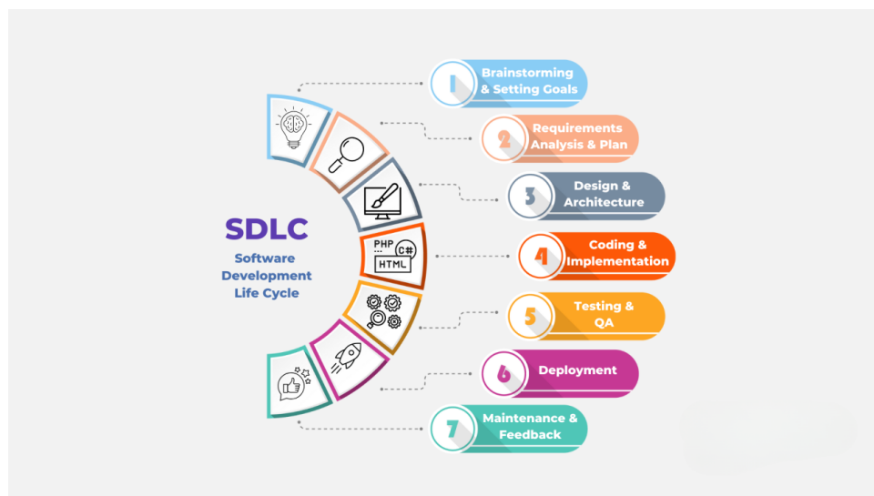
Gambar 2.1: Tahapan SDLC
