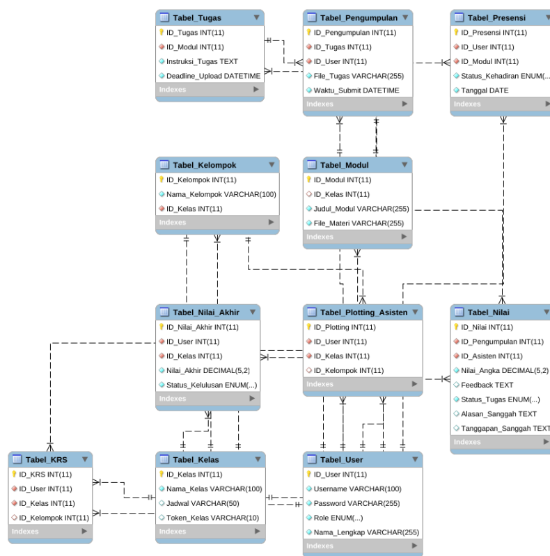
Gambar 4.17: Entity Relationship Diagram (ERD) Sistem EduLab
