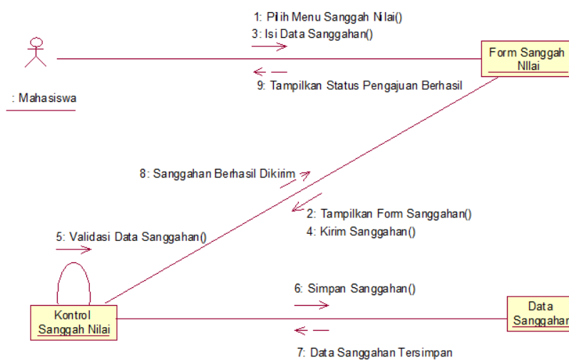
Gambar 4.16: Collaboration Diagram - Skenario Sanggahan Nilai
