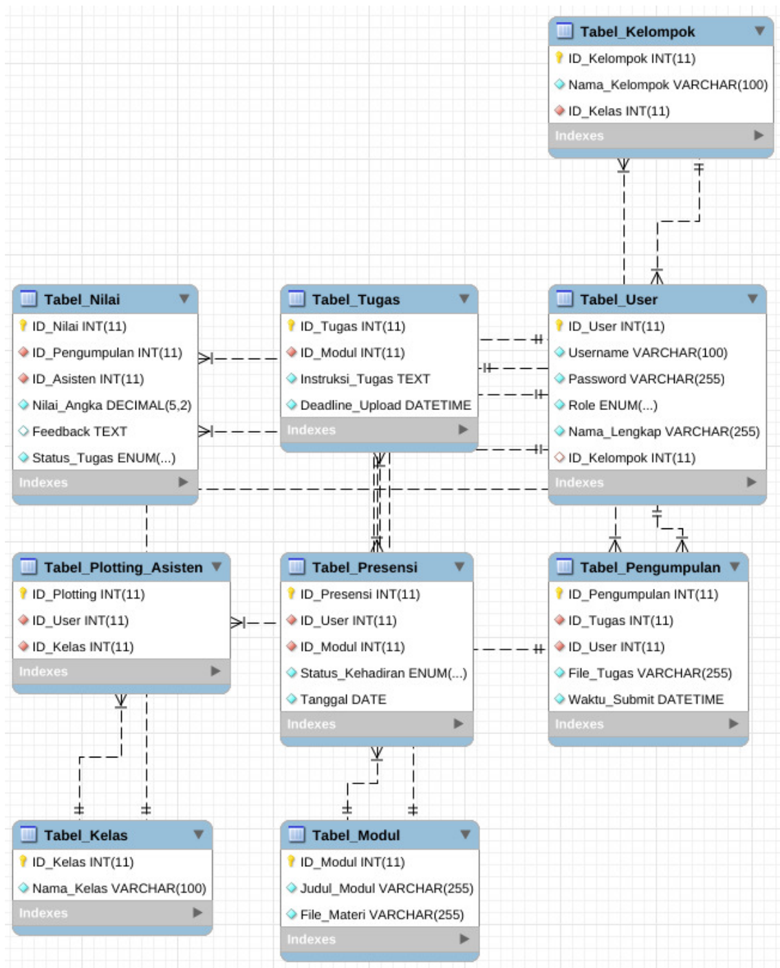
Gambar 4.17: Entity Relationship Diagram (ERD) Sistem EduLab
