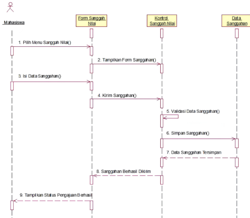
Gambar 4.11: Sequence Diagram - Skenario Sanggah Nilai
