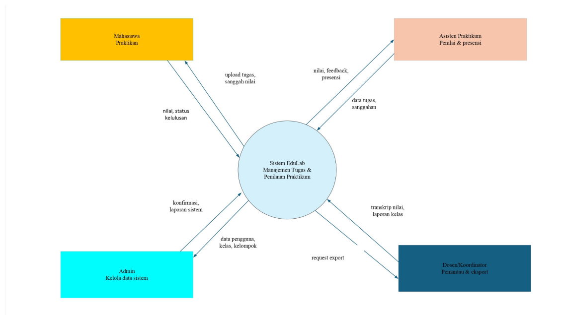
Gambar 4.2: Diagram Konteks Sistem EduLab
