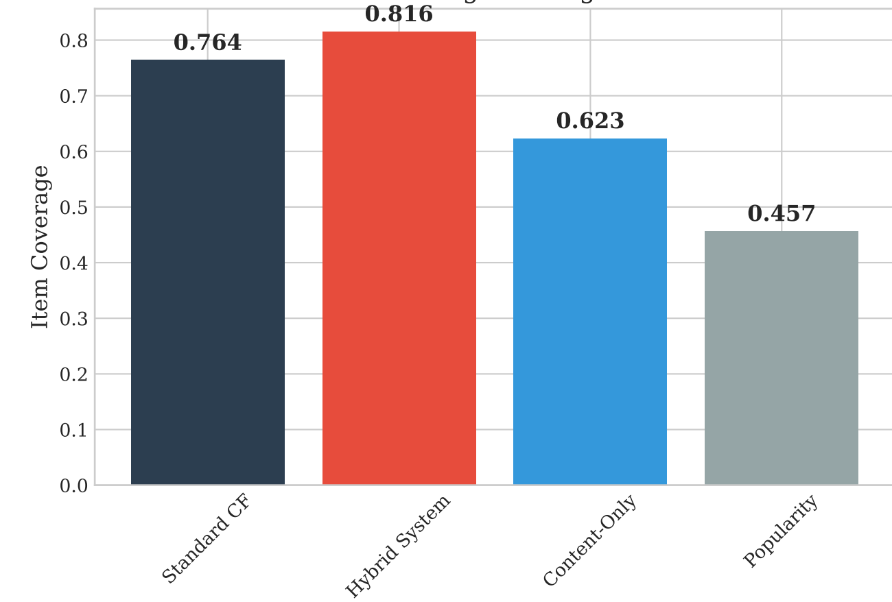
Catalog Coverage
