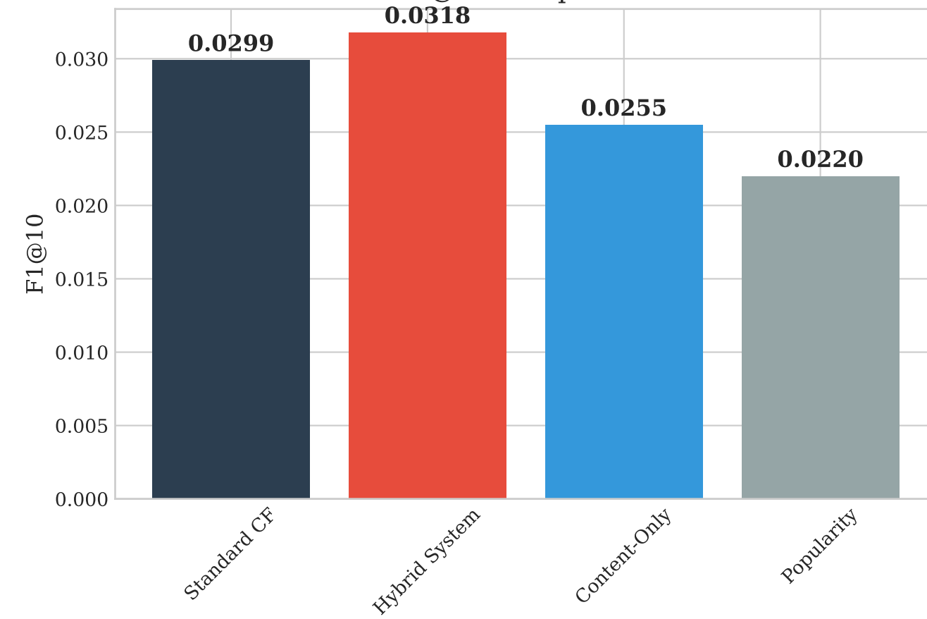
F1@10 Comparison
