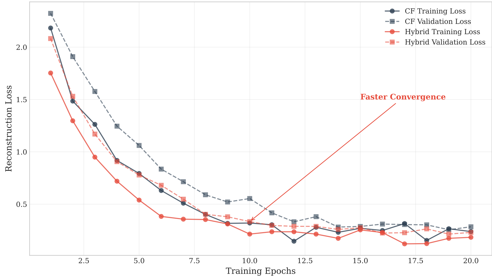
Training Convergence Comparison
