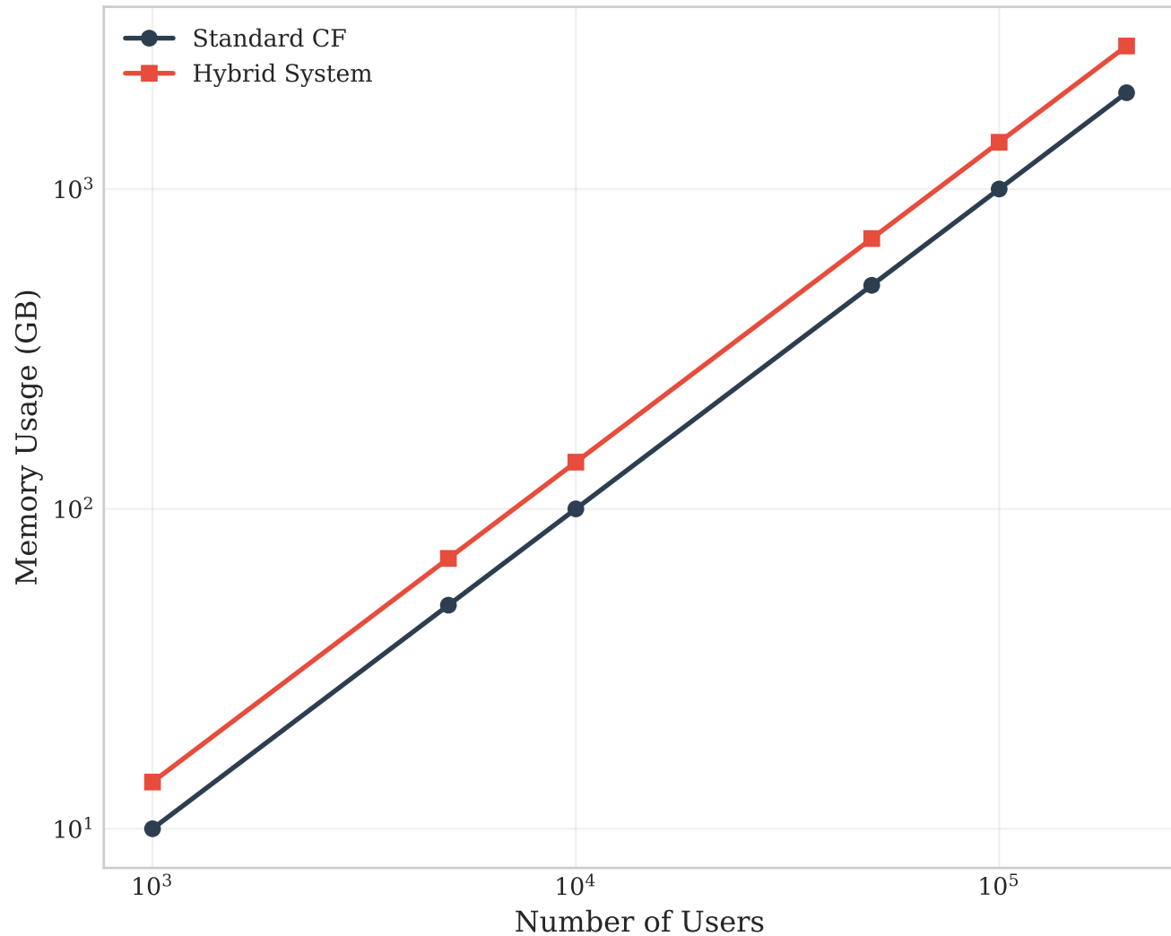
Memory Usage Scalability
