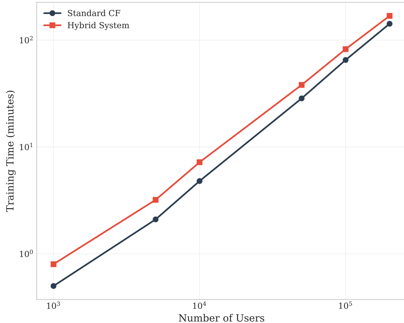
Training Time Scalability
