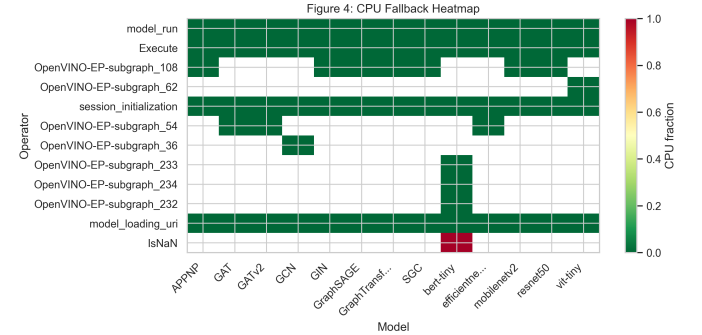
Fig. 4: CPU fallback fraction per operator across models. Most operators run natively on the assigned backend. MPNN and attention-based models trigger toolchain limitations.
