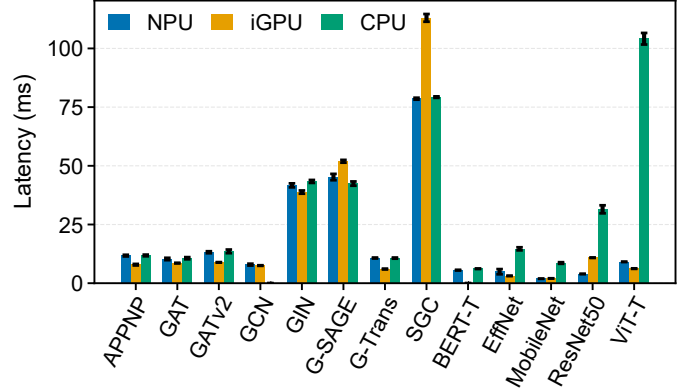
Fig. 1. FP32 latency comparison across CPU, iGPU, and NPU backends. Error bars indicate per-iteration standard deviation. GNNs show near-parity across backends; dense vision models exhibit significant NPU advantage.
