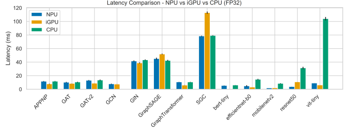
Fig. 1. FP32 latency comparison across CPU, iGPU, and NPU backends. Error bars indicate per-iteration standard deviation. GNNs show near-parity across backends; dense vision models exhibit significant NPU advantage.
