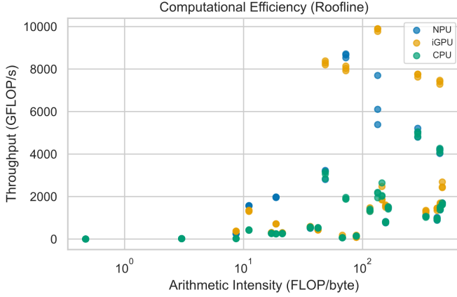
Fig. 5. Computational efficiency (throughput vs. arithmetic intensity). GNNs occupy the memory-bound region (low intensity, low throughput); vision models on NPU achieve higher operational intensity.
