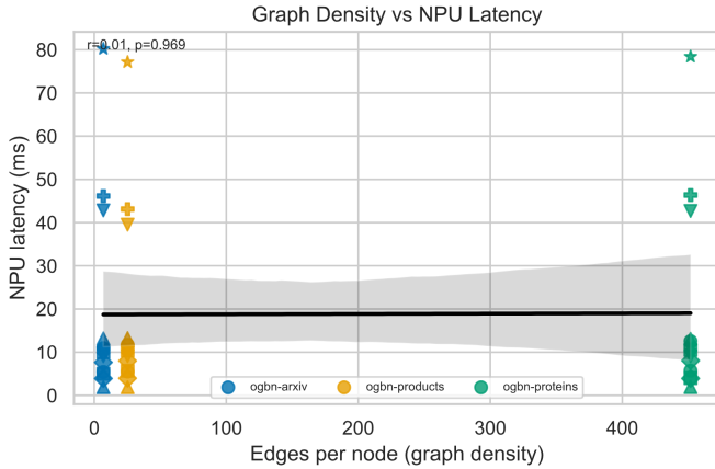
Fig. 6. NPU latency vs. graph density. The flat regression line ( r \approx 0 ) shows no detectable relationship in the evaluated sweep and is consistent with static-shape compilation.
