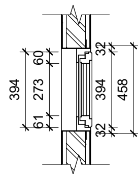
9 DETAIL J4 - SAMPING 1 : 20
