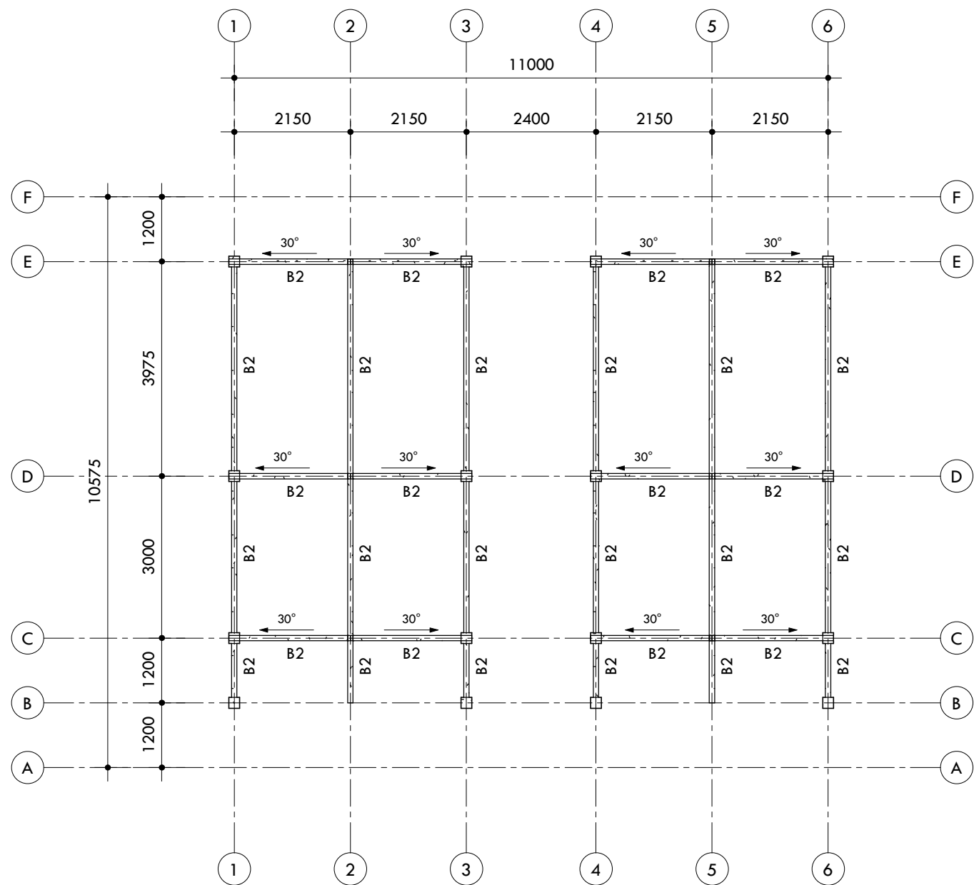
1 DENAH BALOK ELV +6.700 1 : 100
