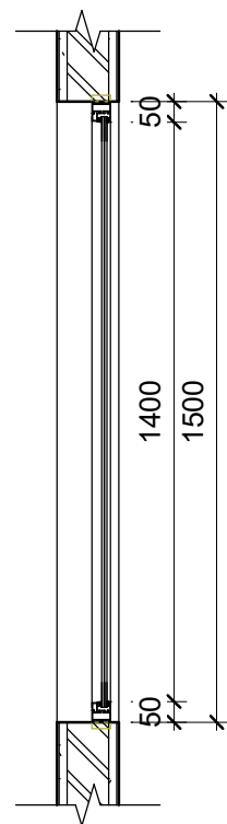
3 DETAIL J2 - SAMPING 1 : 20
