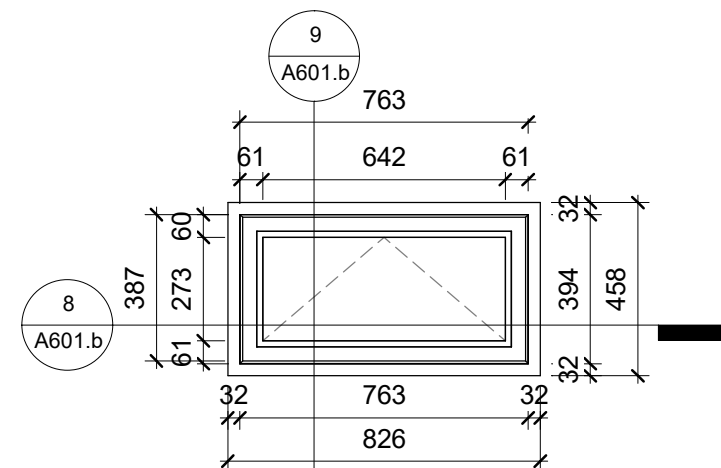
7 DETAIL J4 - DEPAN 1 : 20
