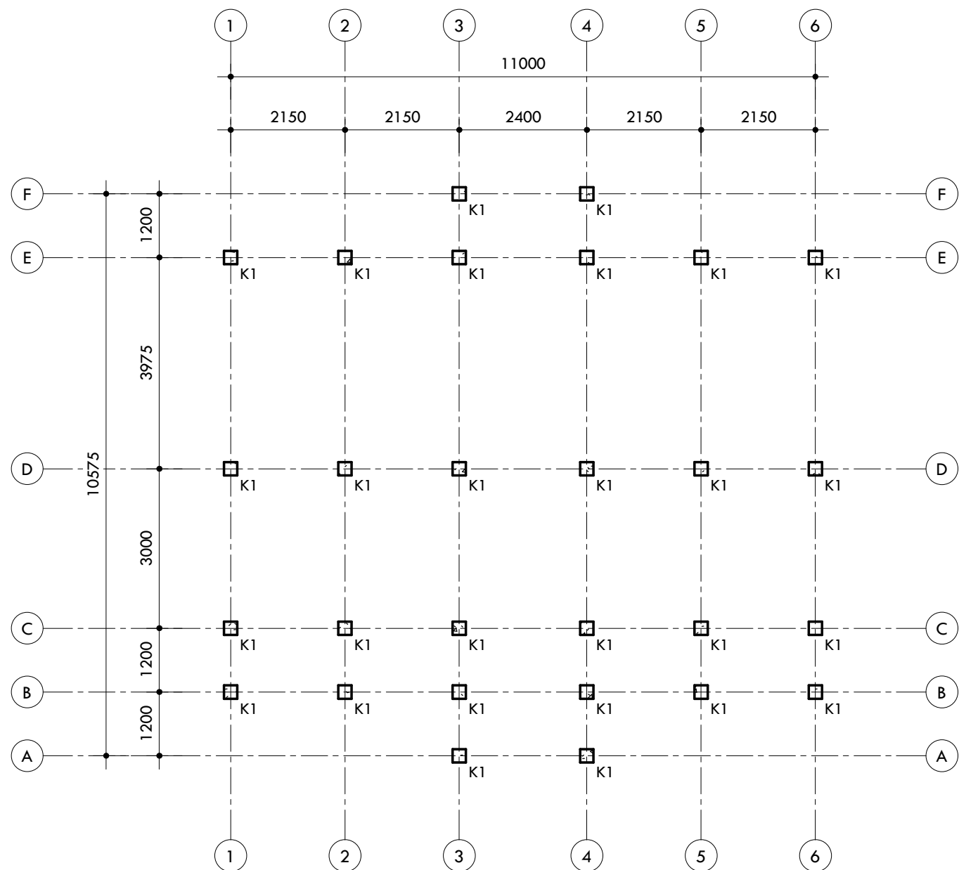
1 DENAH KOLOM PEDESTAL 1 : 100
