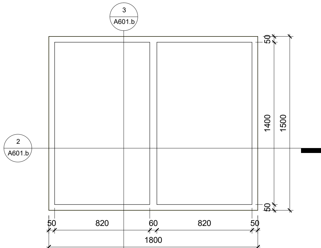
1 DETAIL J2 - DEPAN 1 : 20
