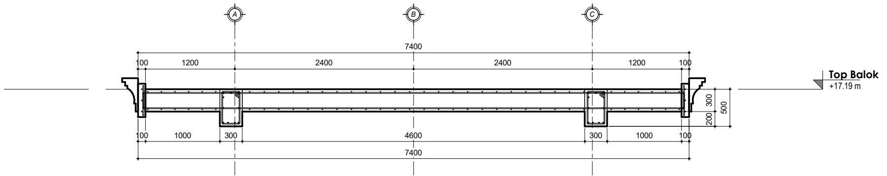
1 Detail Melintang 1 1 : 50
