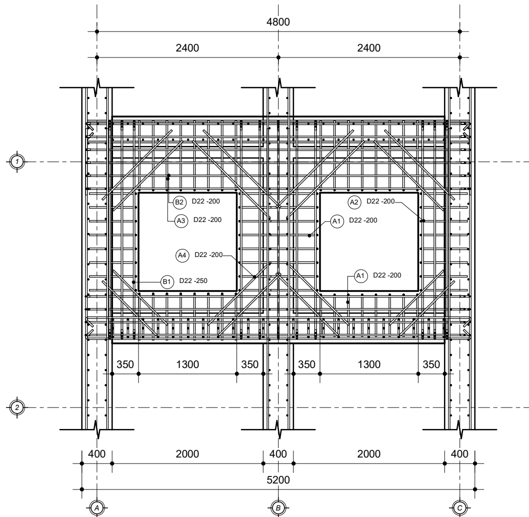
3 Plan View - Slab Pompa 1 : 50
