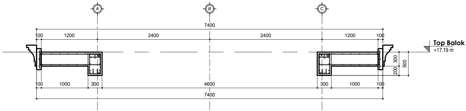
2 Detail Melintang 2 1 : 50
