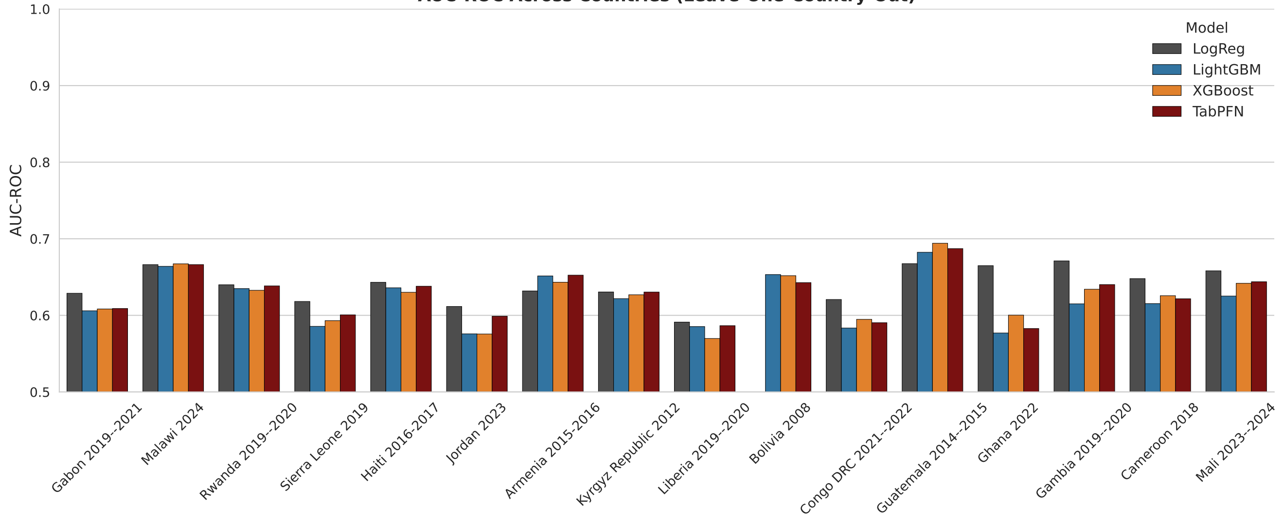
AUC-ROC Across Countries (Leave-One-Country-Out)
