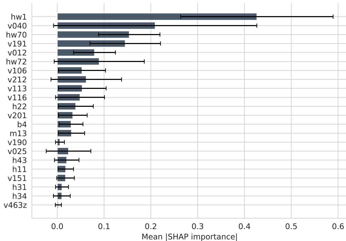
XGBoost
