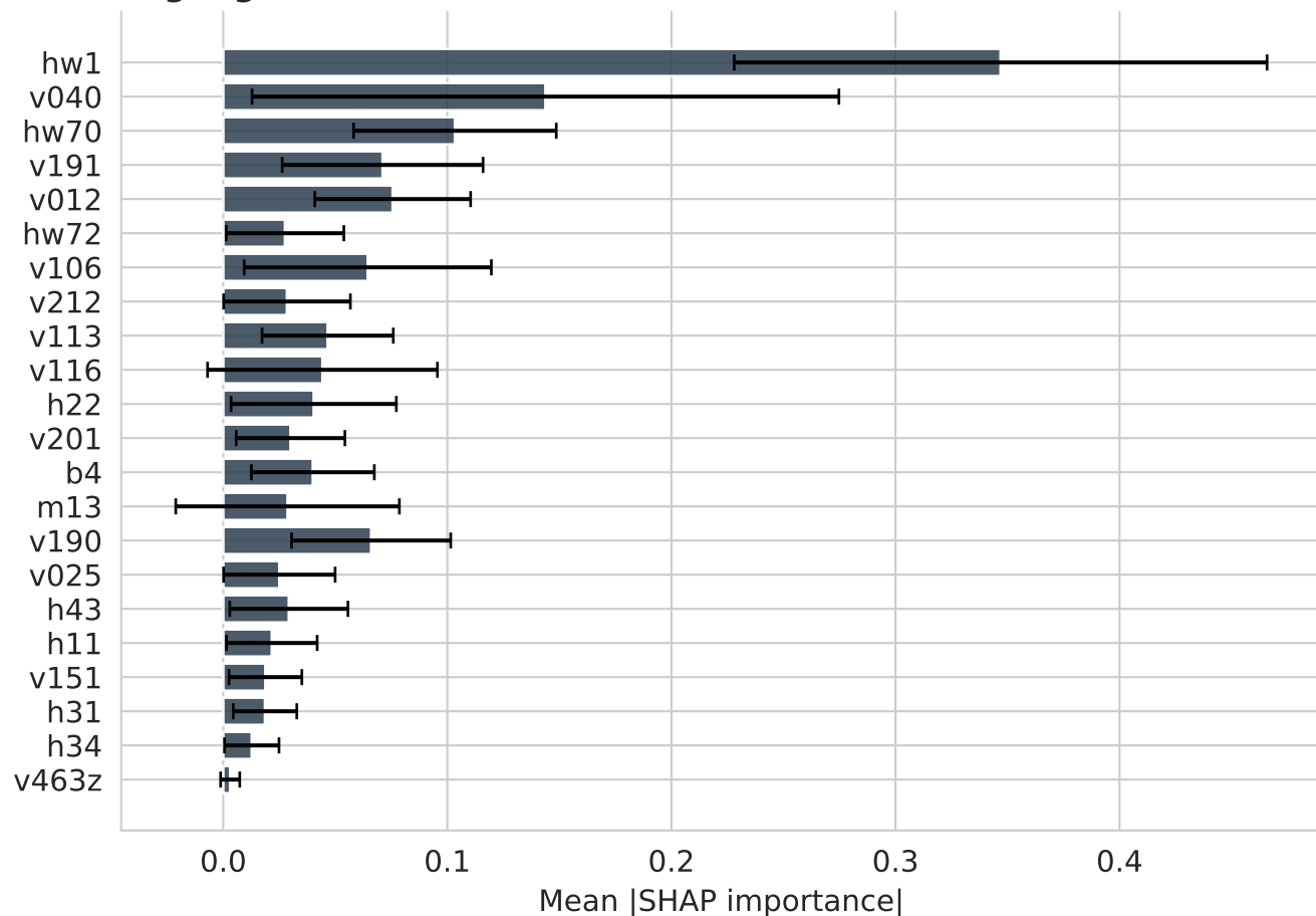
XGBoost
