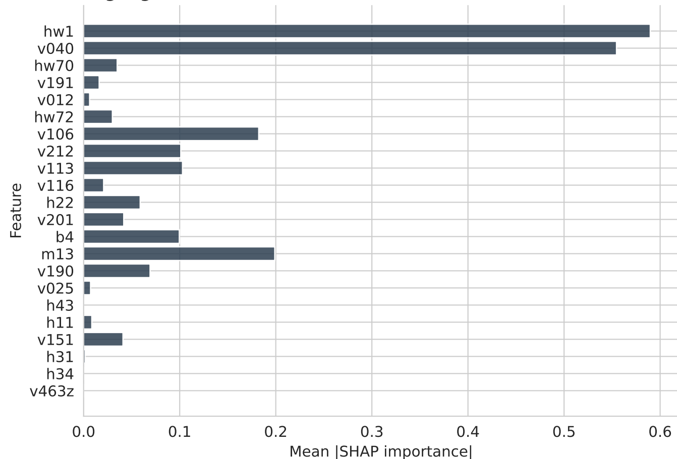
XGBoost
