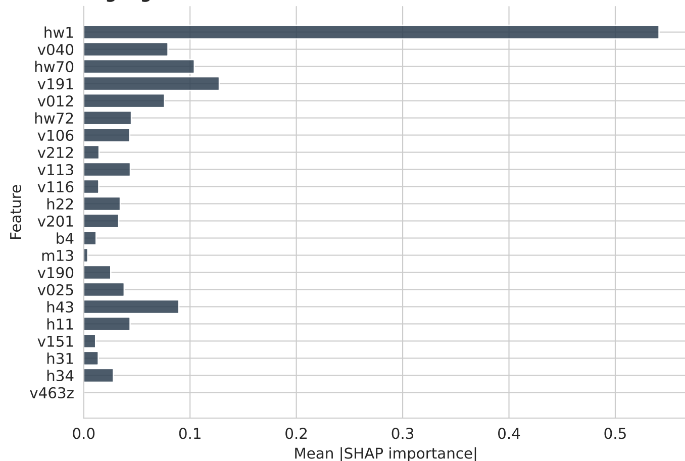
XGBoost
