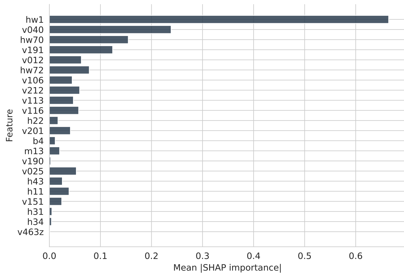
XGBoost
