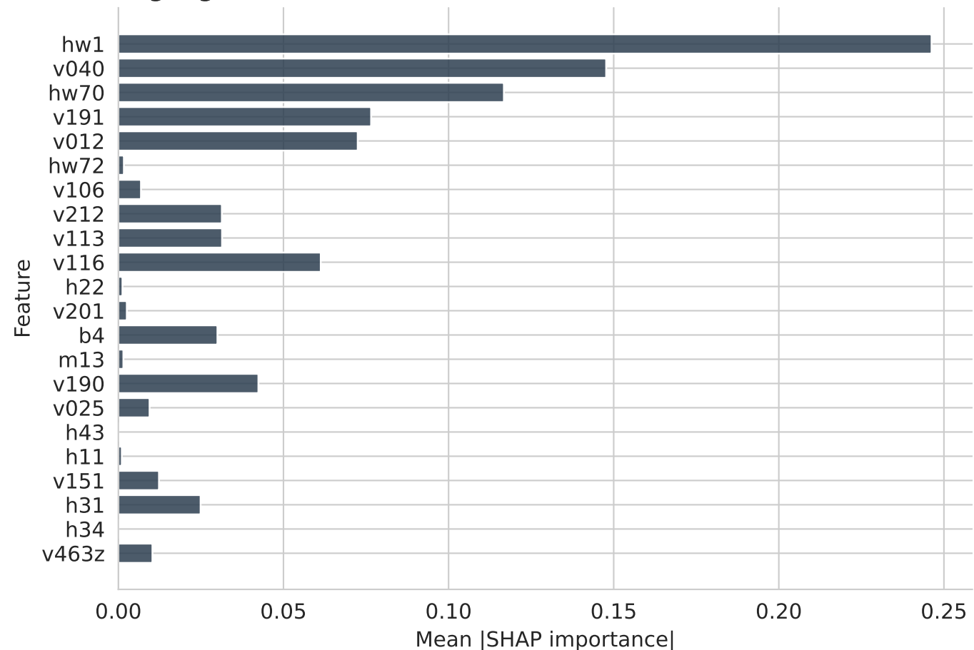
XGBoost
