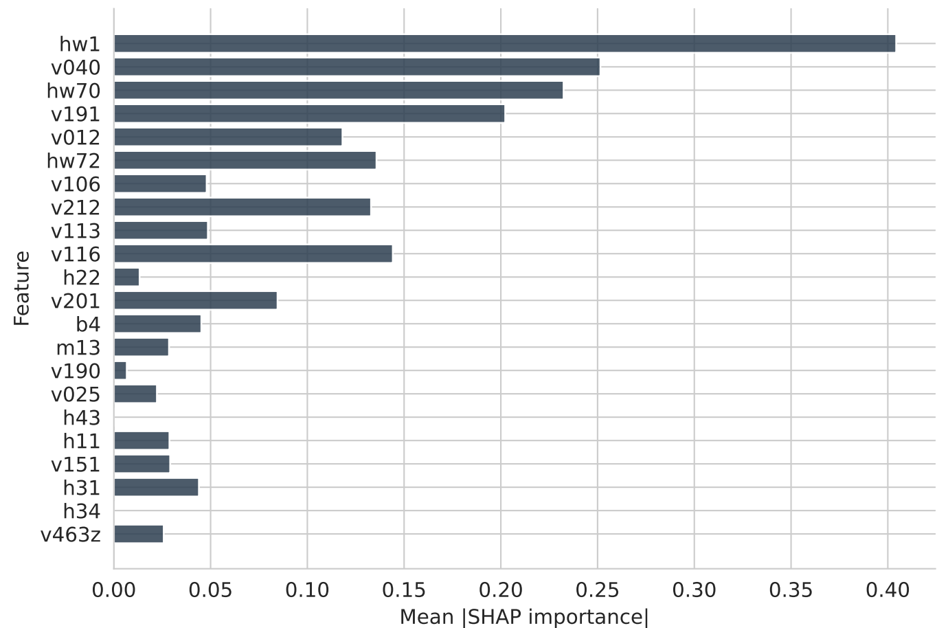
XGBoost
