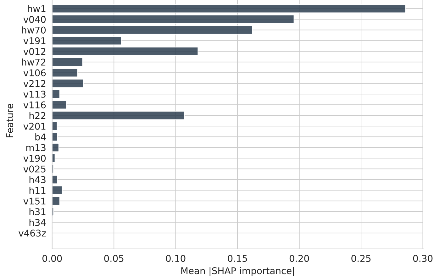
XGBoost
