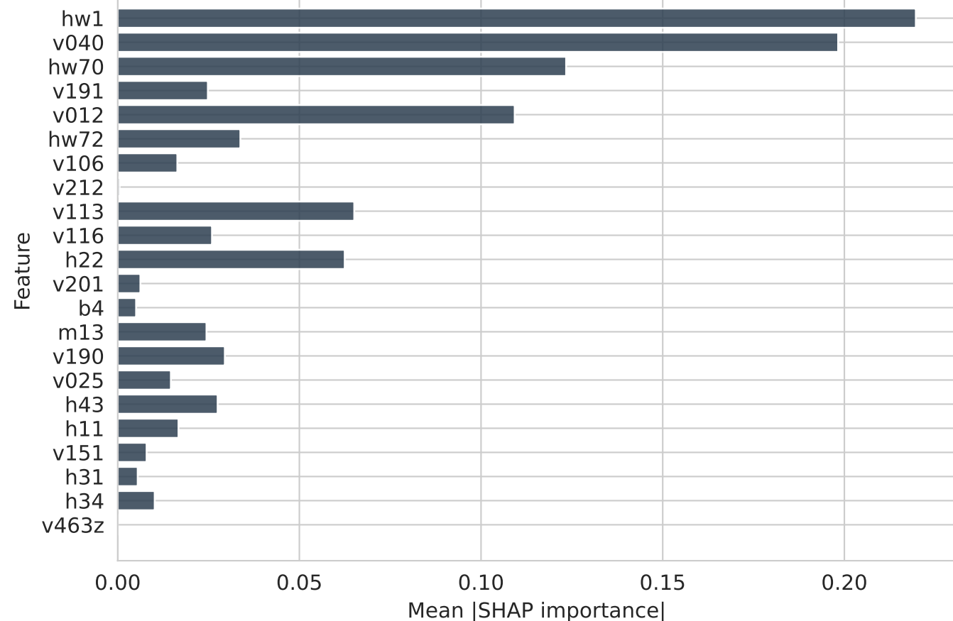
XGBoost
