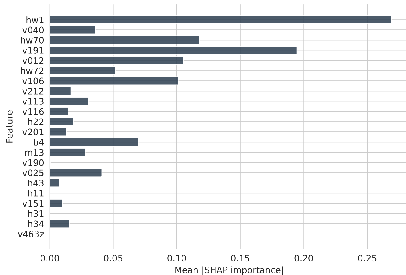
XGBoost
