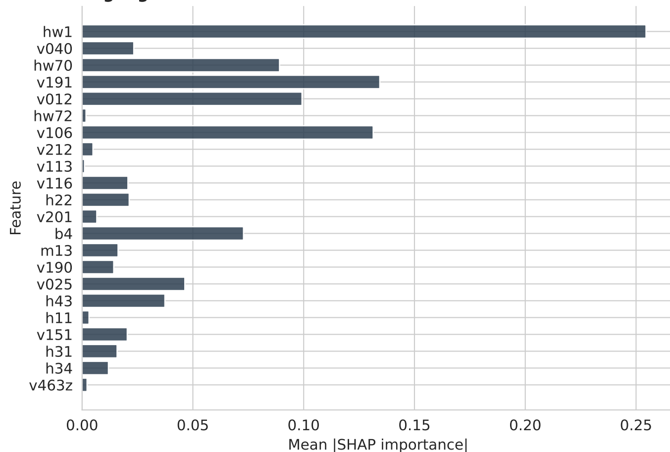
XGBoost
