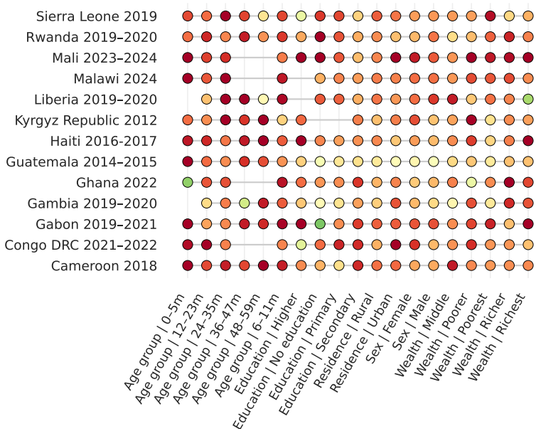
XGBoost
