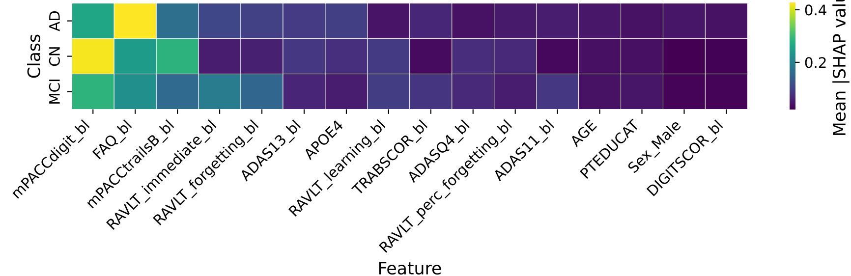
Per-Class Feature Importance (SHAP)
