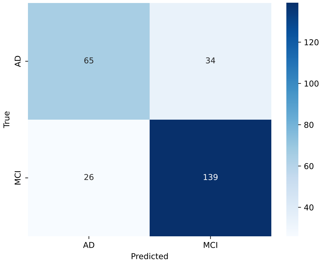
Confusion Matrix — TabularClassifier (Test Set)
