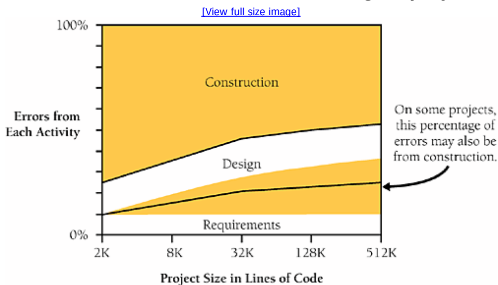
Figure 22-2. As the size of the project increases, the proportion of errors committed during construction decreases. Nevertheless, construction errors account for 45–75 % of all errors on even the largest projects
