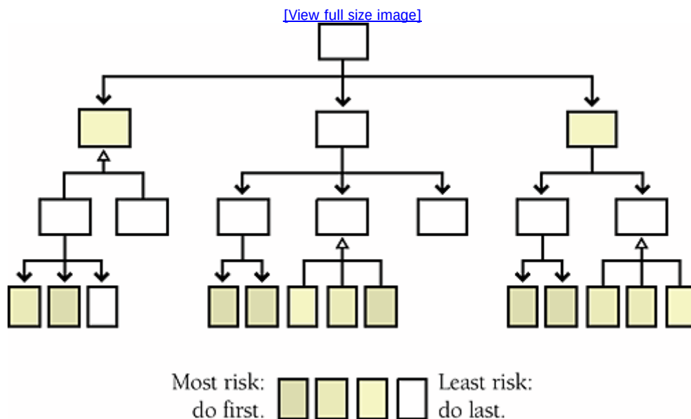
Figure 29-10. In risk-oriented integration, you integrate classes that you expect to be most troublesome first; you implement easier classes later
