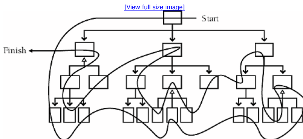
Figure 29-9. In sandwich integration, you integrate top-level and widely used bottom-level classes first and you save middle-level classes for last
