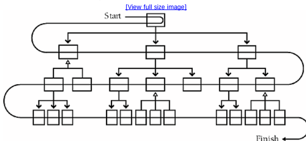
Figure 29-5. In top-down integration, you add classes at the top first, at the bottom last
