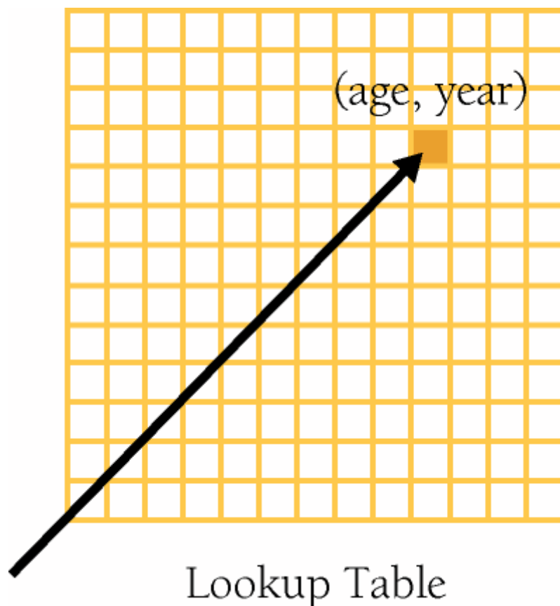
Figure 18-1. As the name suggests, a direct-access table allows you to access the table element you're interested in directly
