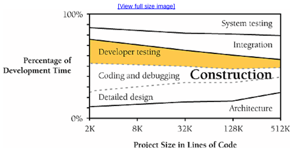
Figure 22-1. As the size of the project increases, developer testing consumes a smaller percentage of the total development time. The effects of program size are described in more detail in Chapter 27, "How Program Size Affects Construction."
