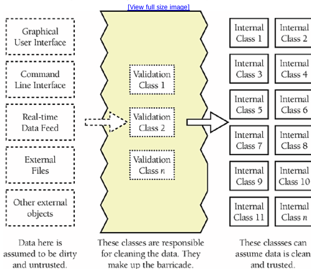
Figure 8-2. Defining some parts of the software that work with dirty data and some that work with clean data can be an effective way to relieve the majority of the code of the responsibility for checking for bad data
