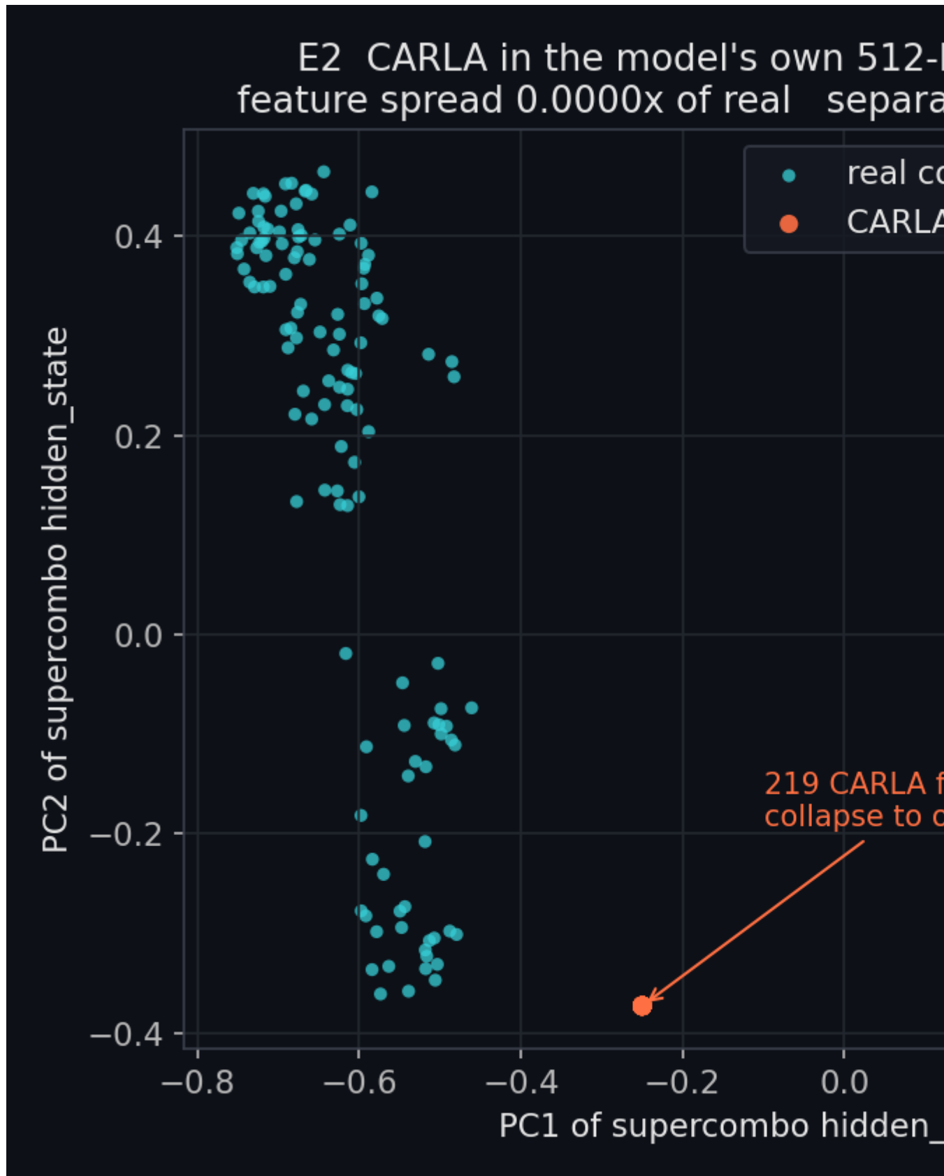
E2: projected 512-D recurrent feature space. Real-driving states spread out; CARLA states freeze to a single point.
