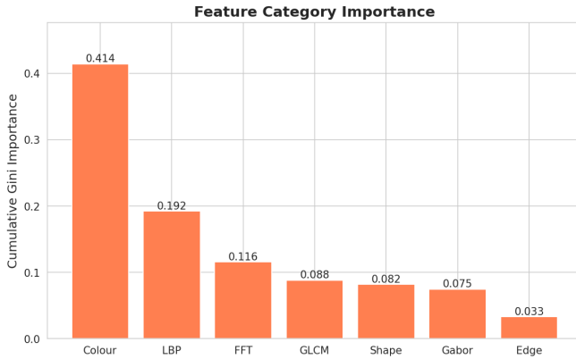
Fig. 5. Cumulative Gini importance of handcrafted feature categories (Random Forest on handcrafted-only features).
