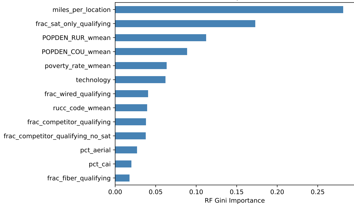
Feature Importances
