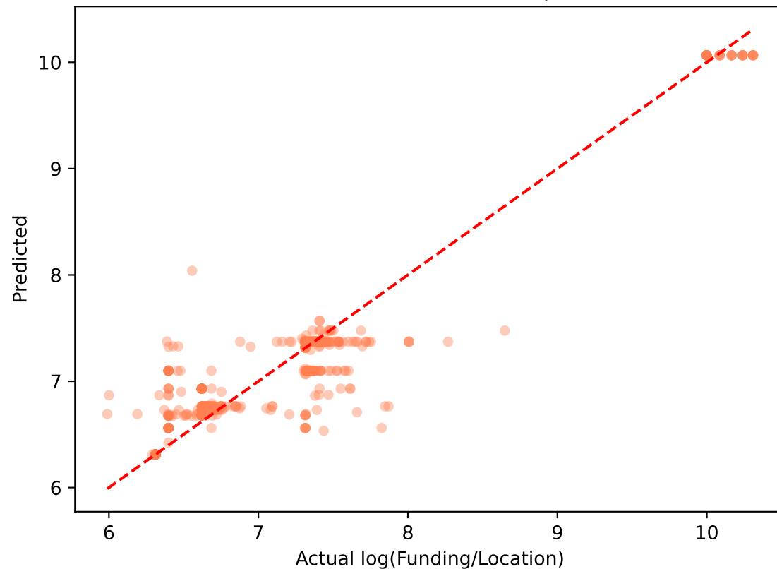
Satellite/LEO (n=1996, 5 feat) | R^2=0.894
