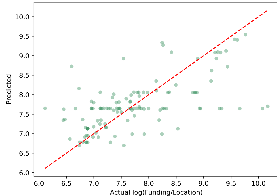
Fixed Wireless (n=410, 5 feat) | R^2=0.358
