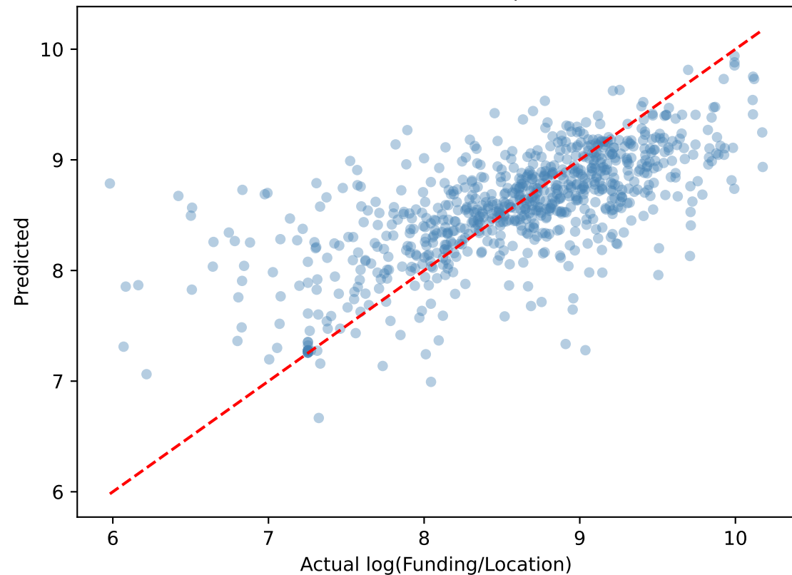
Fiber (n=2569, 10 feat) | R^2=0.464
