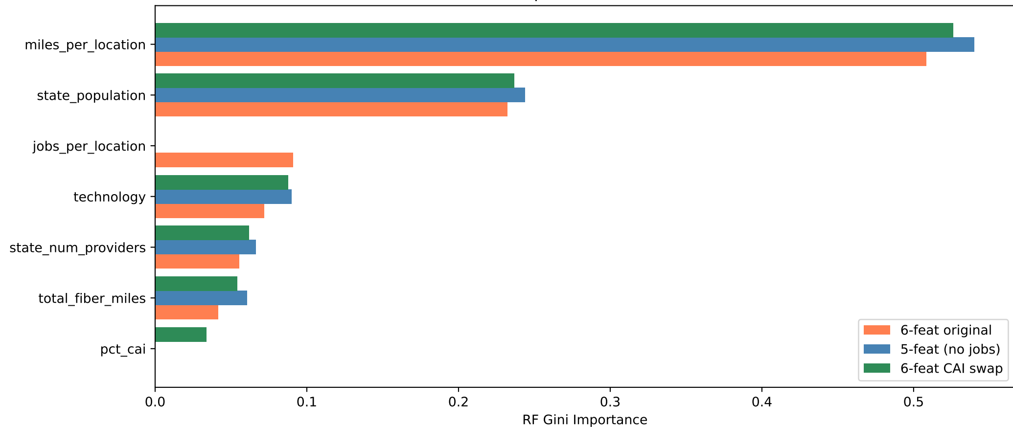
Feature Importance Across Models
