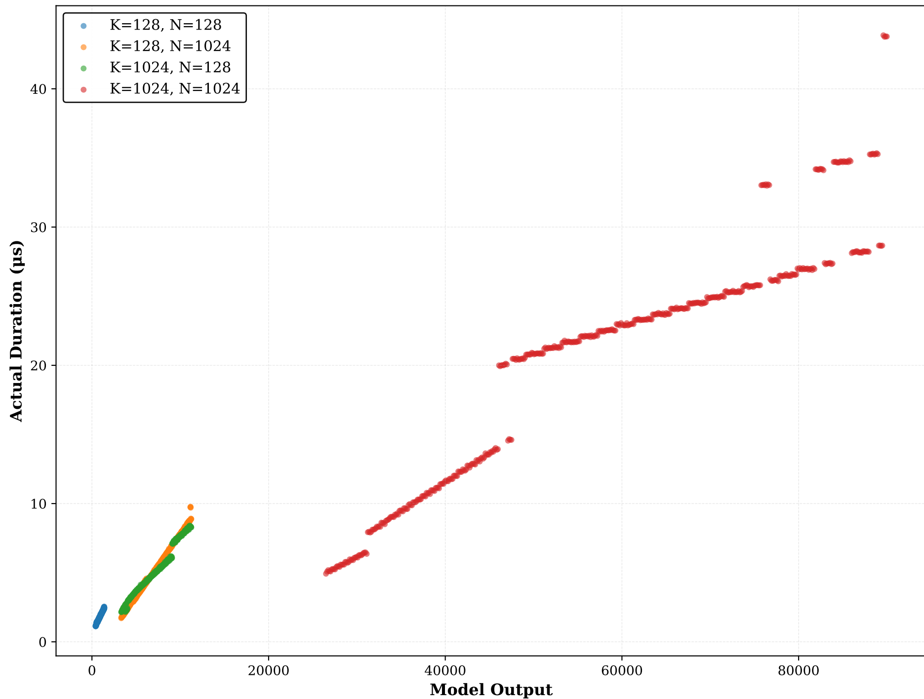
Model Output vs Actual Duration for Different GEMM Configurations
