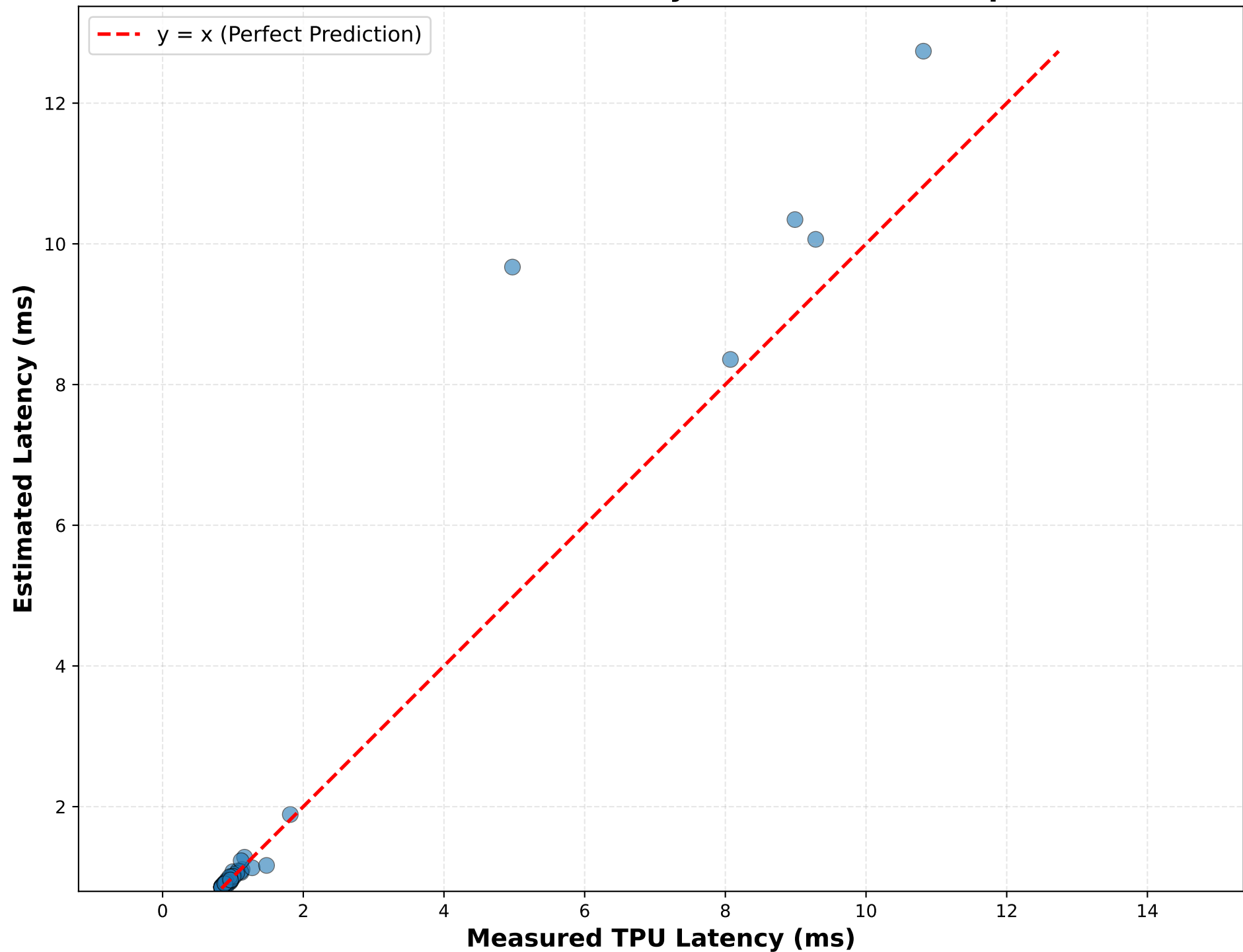
Estimated vs Measured Latency for Elementwise Operations
