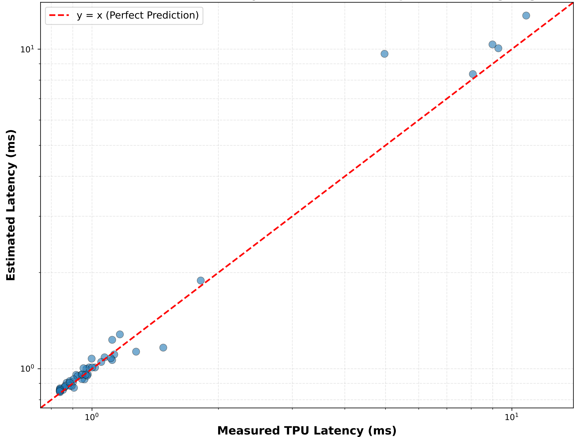
Estimated vs Measured Latency for Elementwise Operations (Log-Log Scale)
