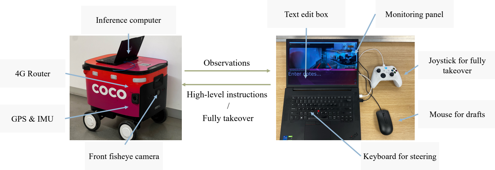
(a) COCO wheeled delivery robots
