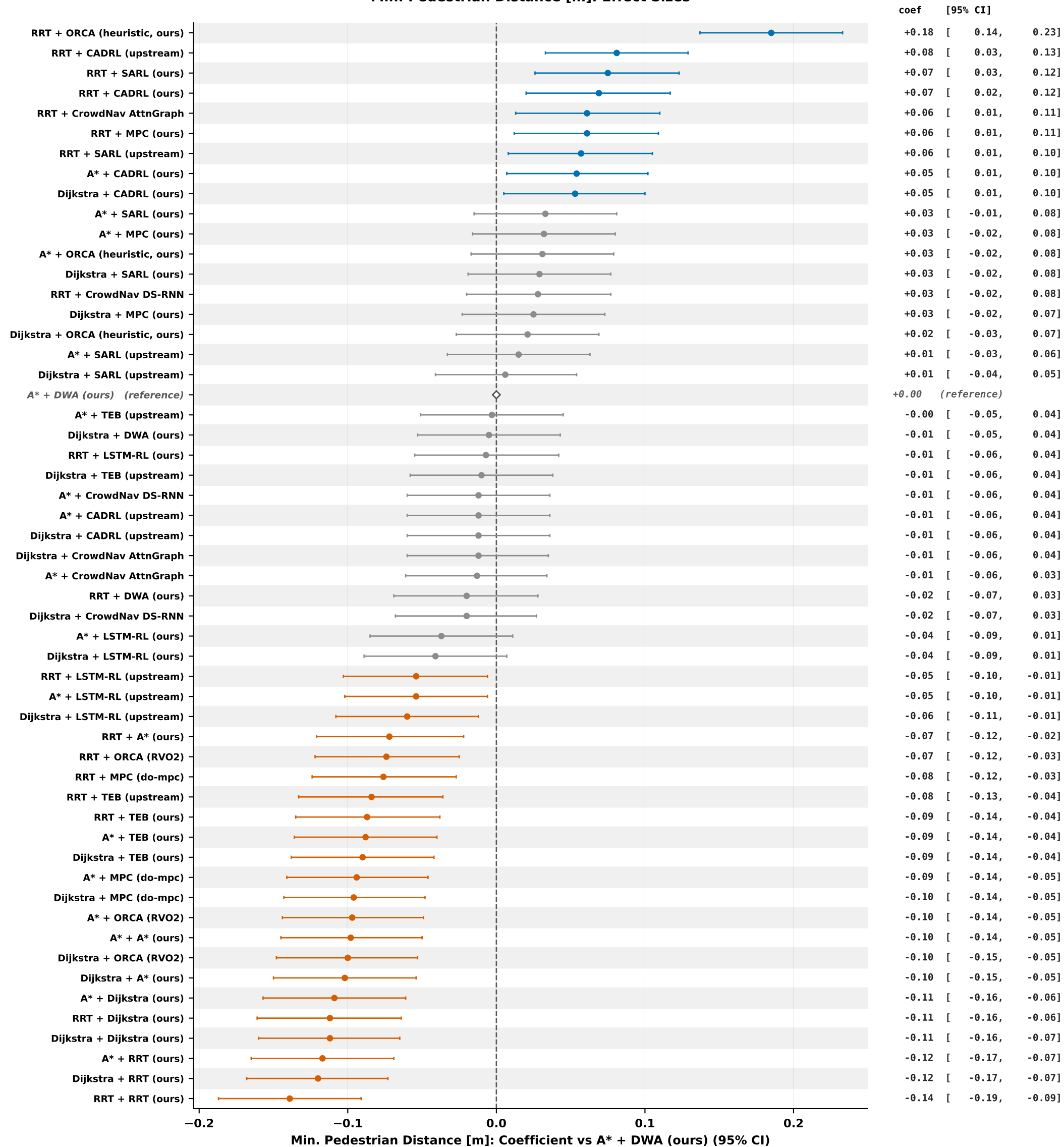
Min. Pedestrian Distance [m]: Effect Sizes
