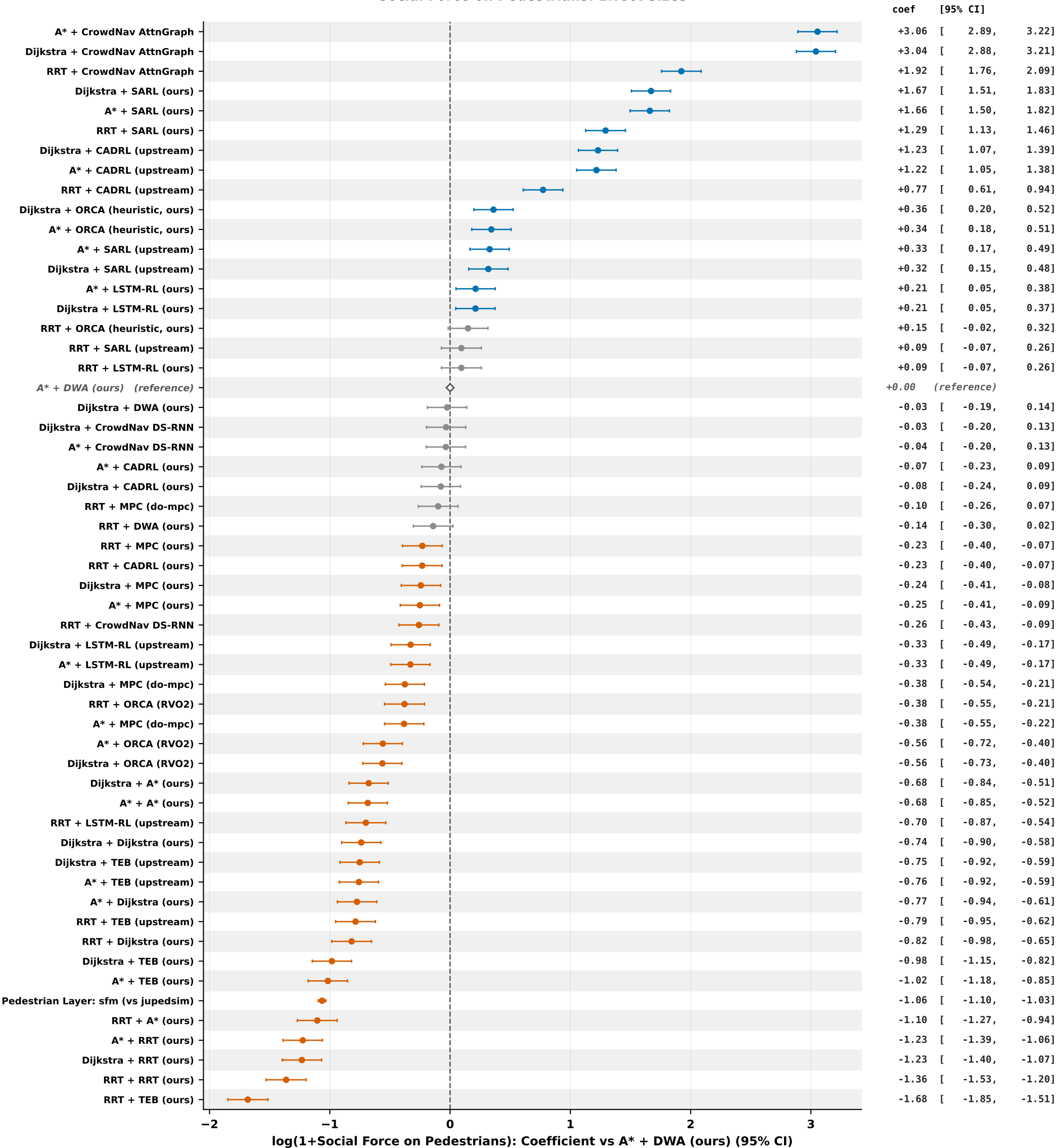
Social Force on Pedestrians: Effect Sizes
