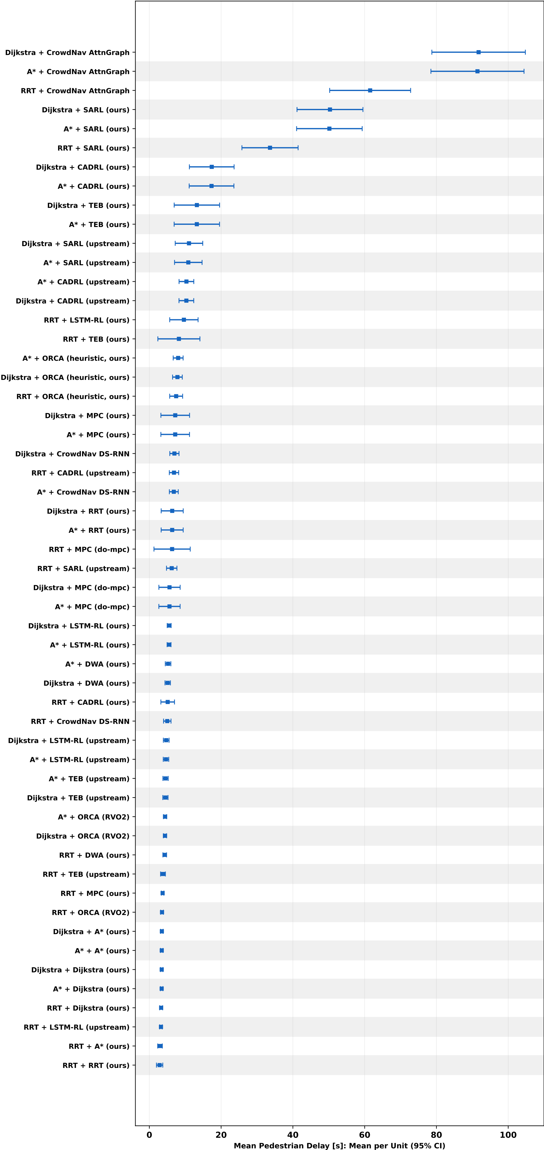
Mean Pedestrian Delay [s]: Mean per Unit (95% CI)
