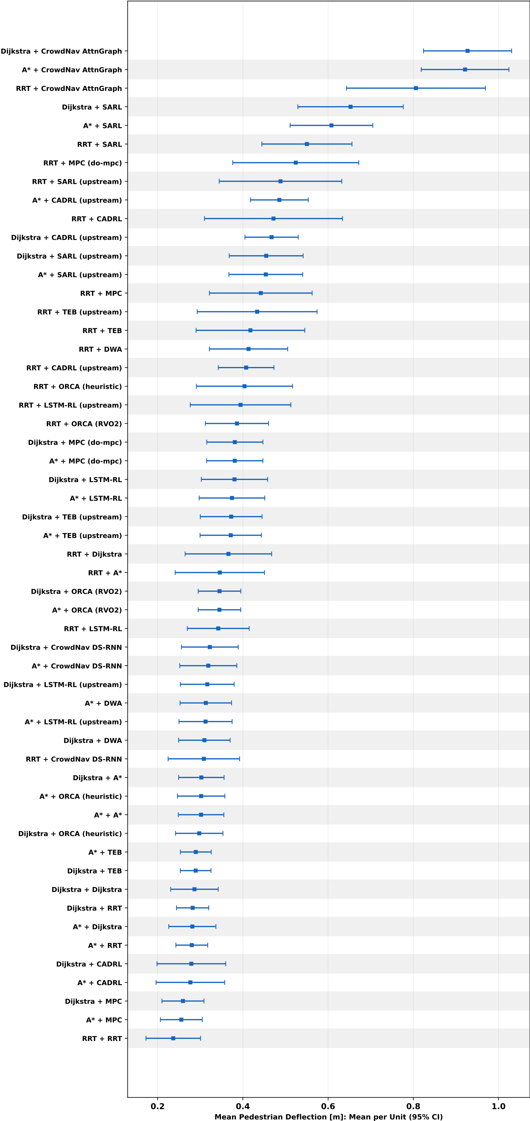
Mean Pedestrian Deflection [m]: Mean per Unit (95% CI)
