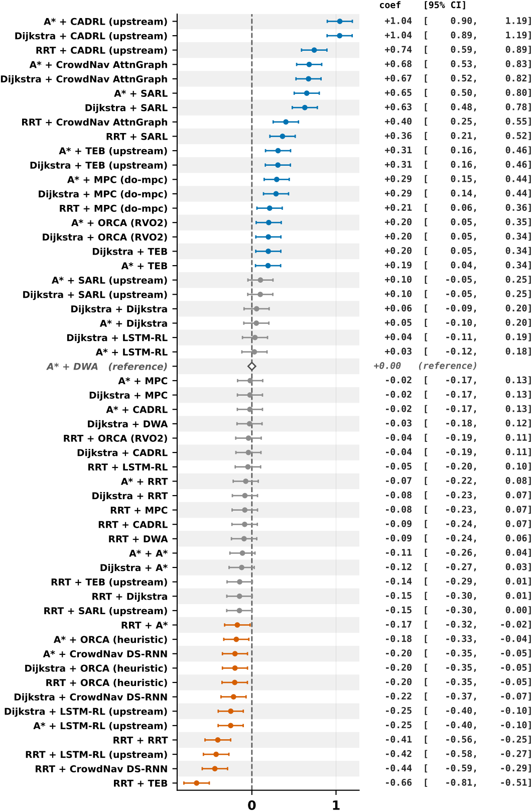
log(1+Personal-Space Intrusion [s]): Coefficient vs A* + DWA (95% CI)
