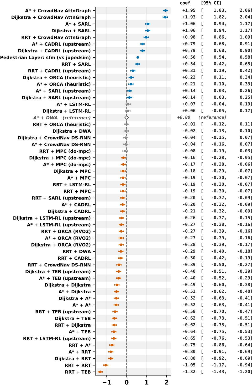
log(1+Social Force on Robot): Coefficient vs A* + DWA (95% CI)
