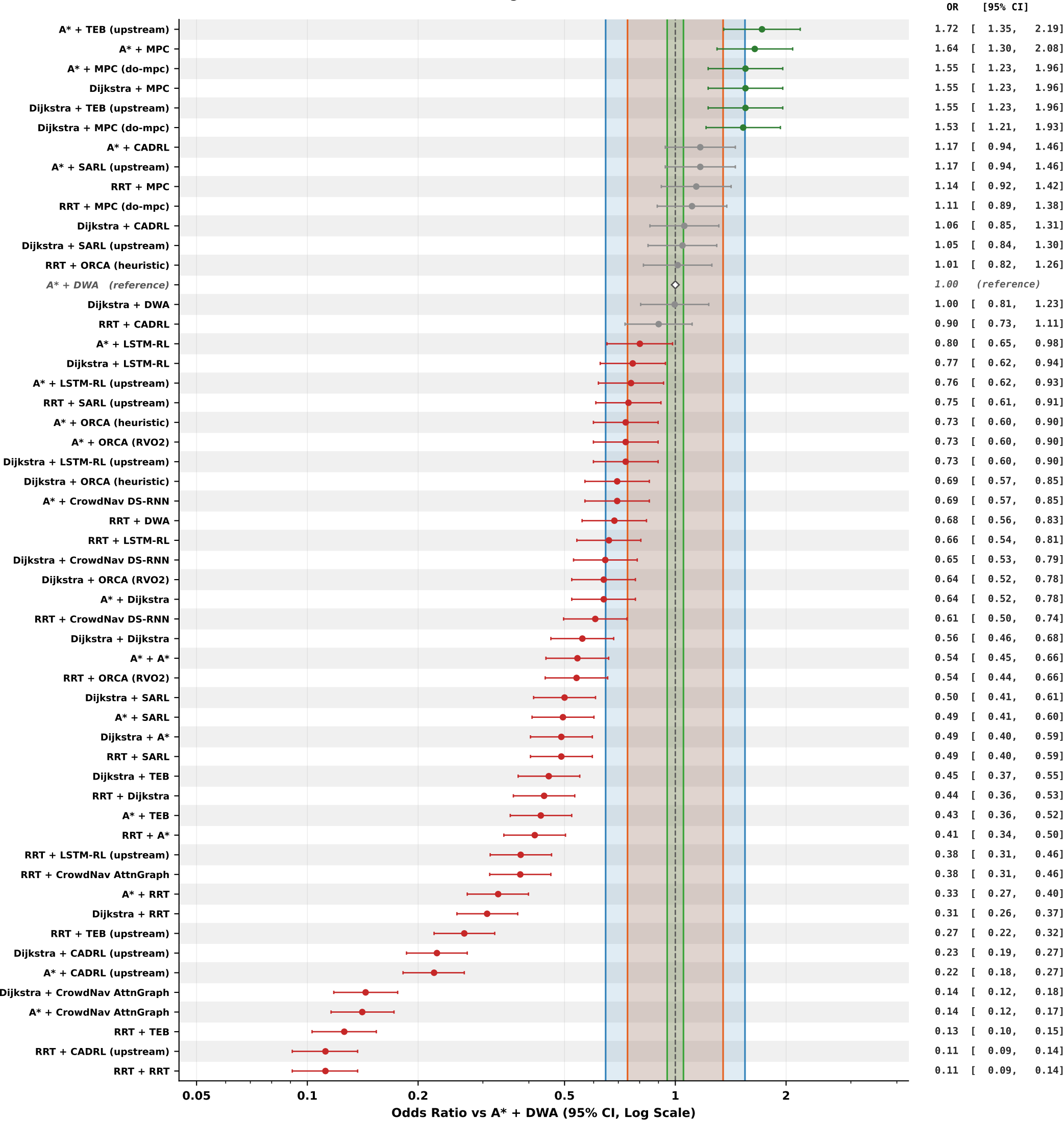
Success: Algorithm Effect Sizes
