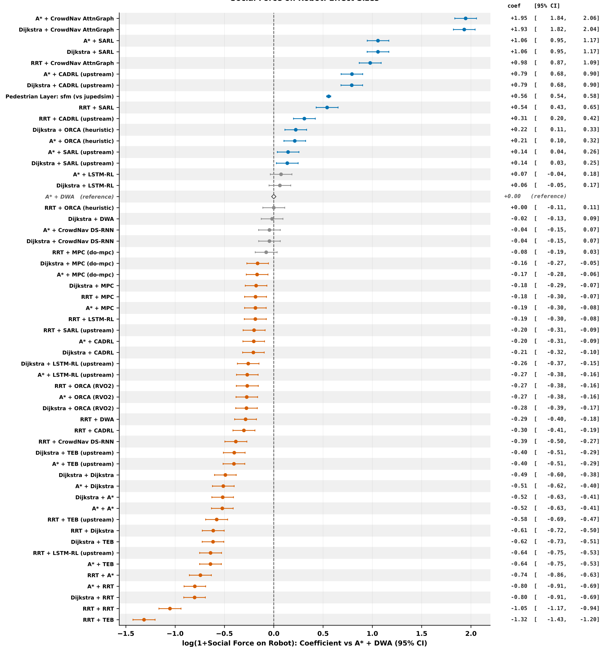
Social Force on Robot: Effect Sizes
