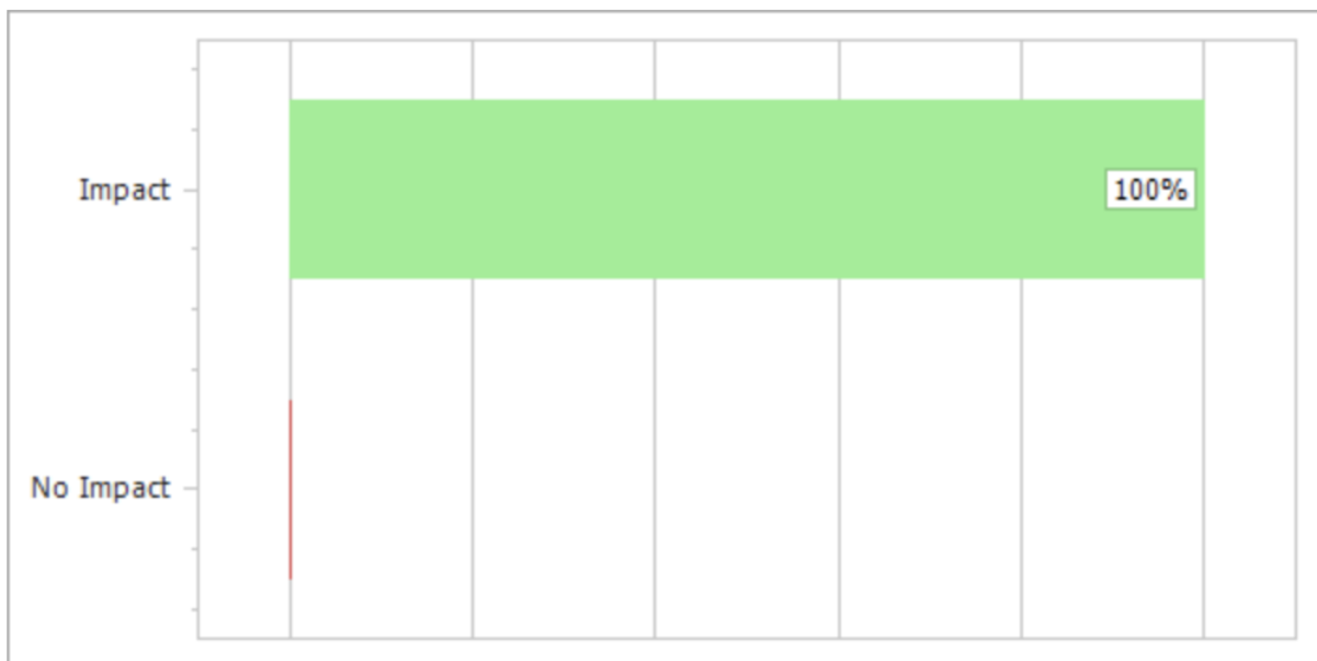
Figure 2: Assignments
