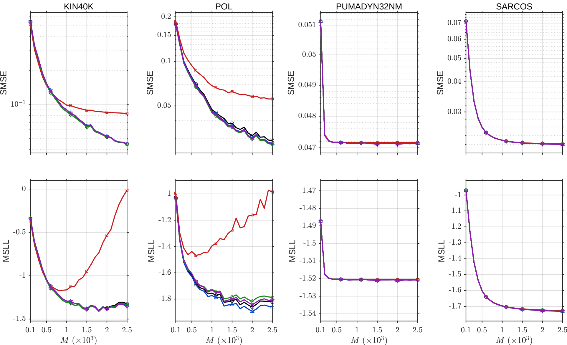
Effect of the Number of Inducing Points under IP-DAC
