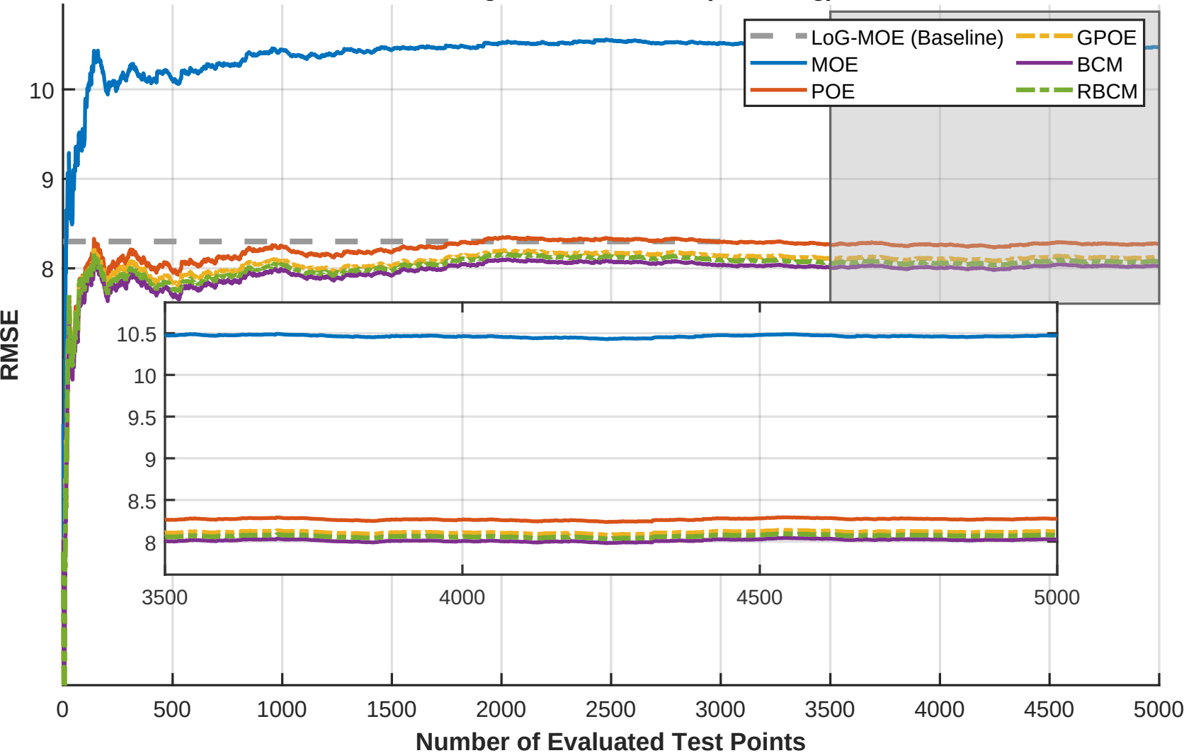
POL - Fig2 IP DAC - RMSE (5 MC Avg)
