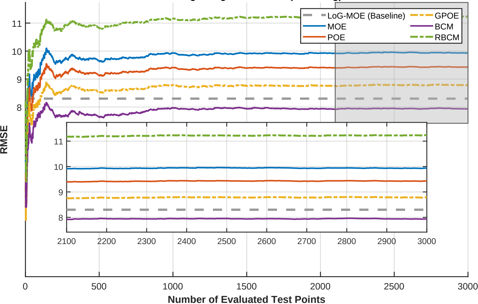
POL - Fig5 Neighbor - RMSE (5 MC Avg)
