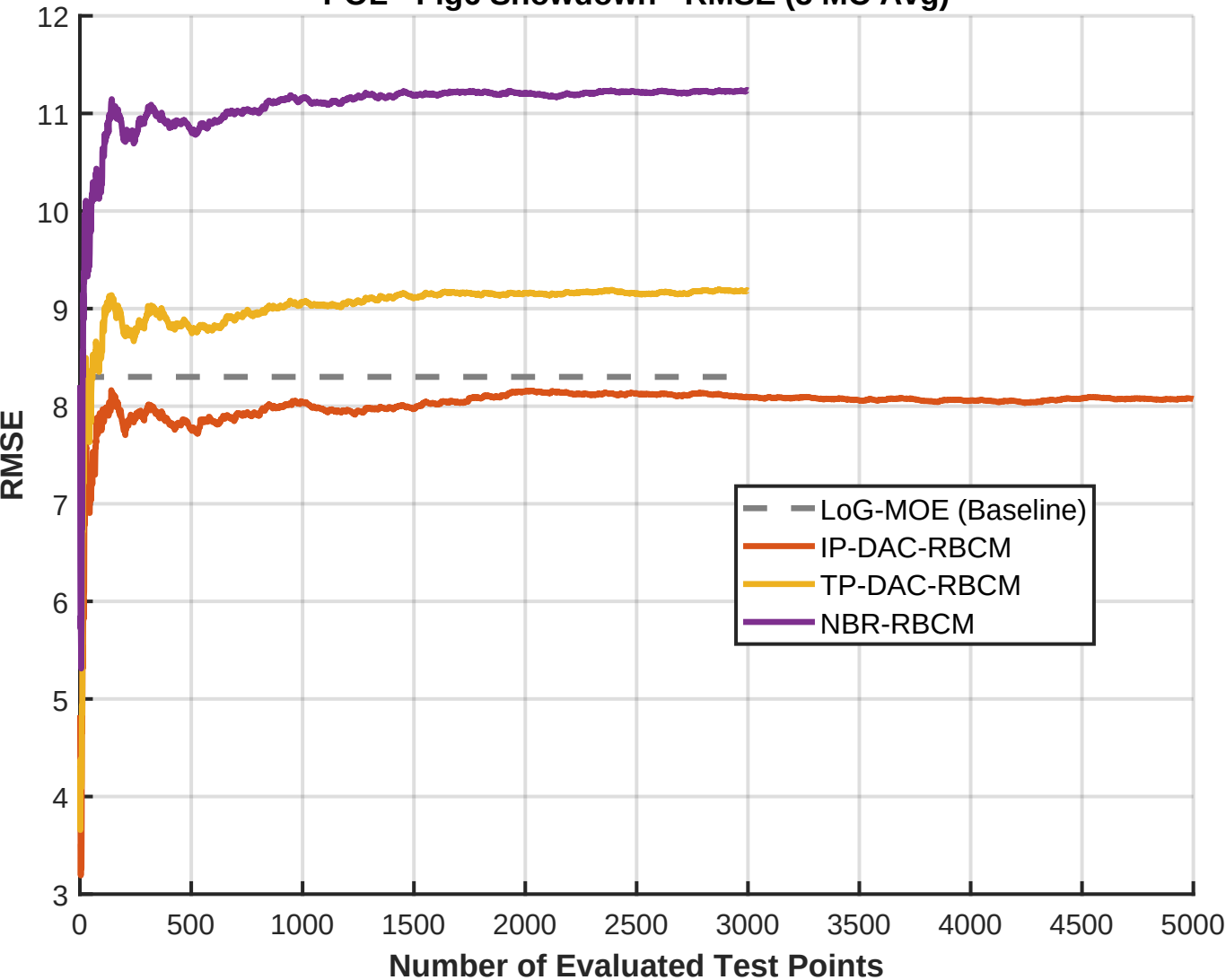
POL - Fig6 Showdown - RMSE (5 MC Avg)
