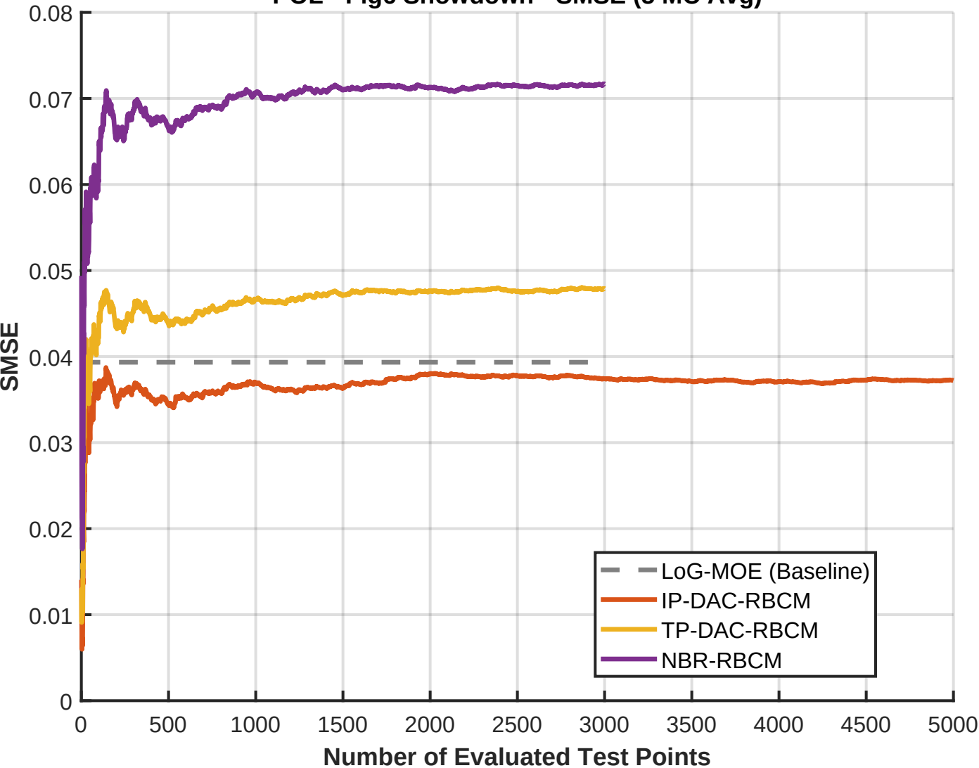
POL - Fig6 Showdown - SMSE (5 MC Avg)
